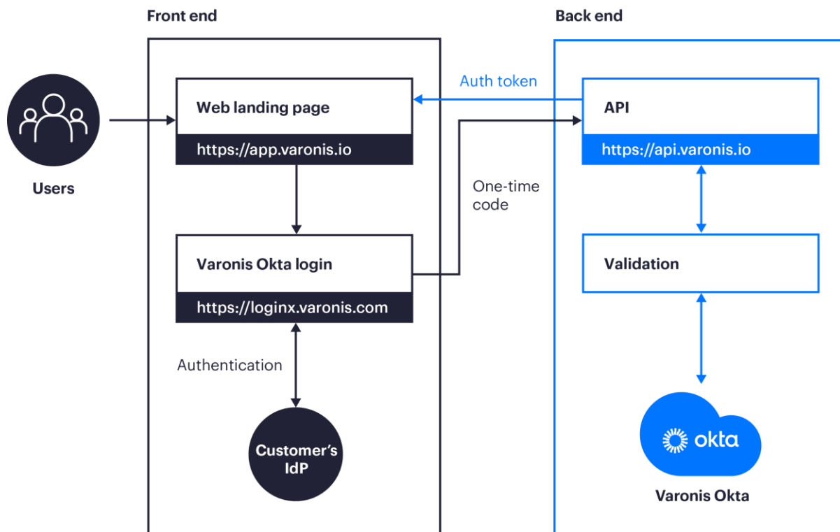
Figure 2: Federated authentication workflow
